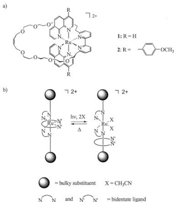
Figure 2. (a) Chemical structures of complexes 1 and 2 . (b) Possible photochemical reaction leading to a rotaxane if bulky stoppers are attached in the 4 positions
