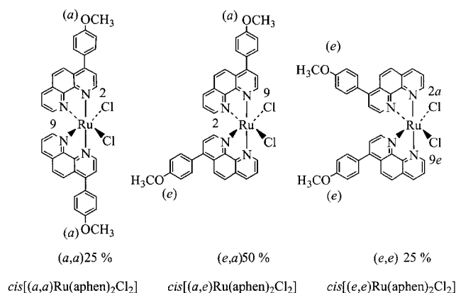
Figure 3. Schematic view of the isomeric complexes for the general species \text{cis-}[\text{Ru}(\text{aphen})_2\text{Cl}_2]^{2+} ( a for axial, e for equatorial)
