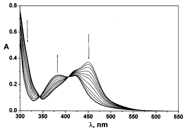
Figure 4. Changes in the electronic absorption spectra of a 2.5 \times 10^{-5} M acetonitrile solution of 1 under irradiation with a 150 W xenon lamp at 404 nm. Spectra are recorded at t = 0, 2, 5, 10, 15, 20, 30, 45, 60, 90, 120 min of irradiation
