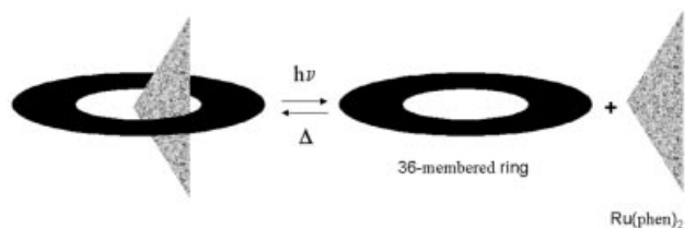
Figure 1. Principle of the photochemically driven motion and the thermal backward reaction
