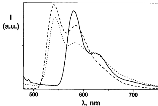
Figure 5. Emission spectra at 77 K of a \text{CH}_3\text{CN} rigid matrix of 1 before (full line, \lambda_{\text{exc}} = 449 nm) and after (dotted line, \lambda_{\text{exc}} = 420 nm) irradiation and of \text{cis-}[\text{Ru}(\text{phen})_2(\text{CH}_3\text{CN})_2]^{2+} (dashed line, \lambda_{\text{exc}} = 420 nm). O. D. = 0.5 for all samples at the excitation wavelength
